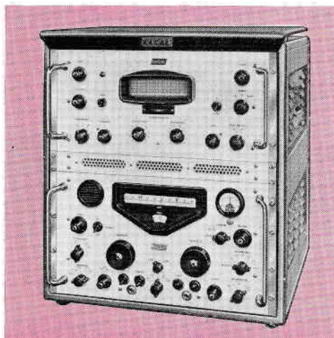
The photograph shows the RA.81 Panoramic Receiver with the RA.66A Panoramic Adaptor. The latter will be replaced by the RA.66B as described above.
